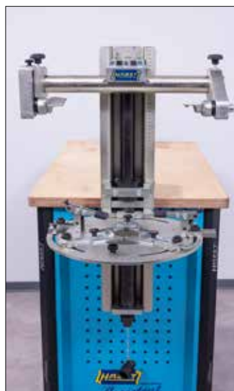
Federspanner 4903/4
